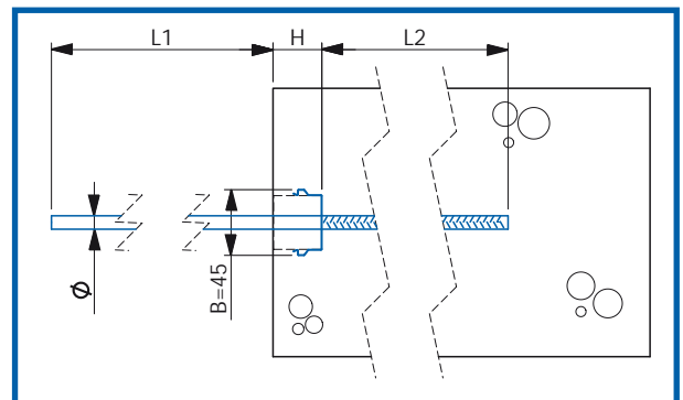
Picture 4. TSK and TSA dimensions [mm]
