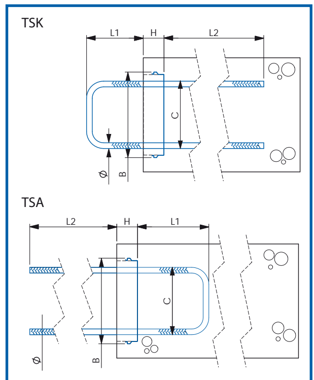
Picture 4. TSK and TSA dimensions [mm]
